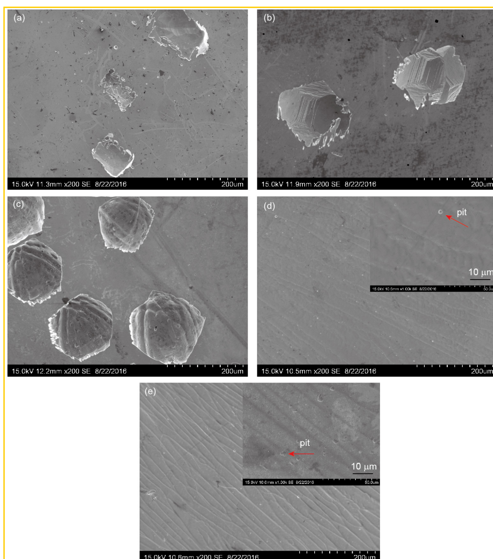
Figure 2 (Color online) The corroded surfaces of alloys in 0.1 M NaCl. (a) Ni; (b) NiCo; (c) NiCoFe; (d) NiCoCr; (e) NiCoCrFe
