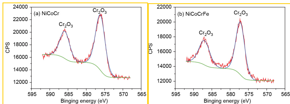
Figure 6 (Color online) The XPS spectra of Cr for NiCoCr and NiCoCrFe in 0.1 M NaCl. (a) NiCoCr; (b) NiCoCrFe
