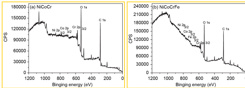
Figure 5 The XPS survey spectra of NiCoCr and NiCoCrFe in 0.1 M NaCl. (a) NiCoCr; (b) NiCoCrFe
