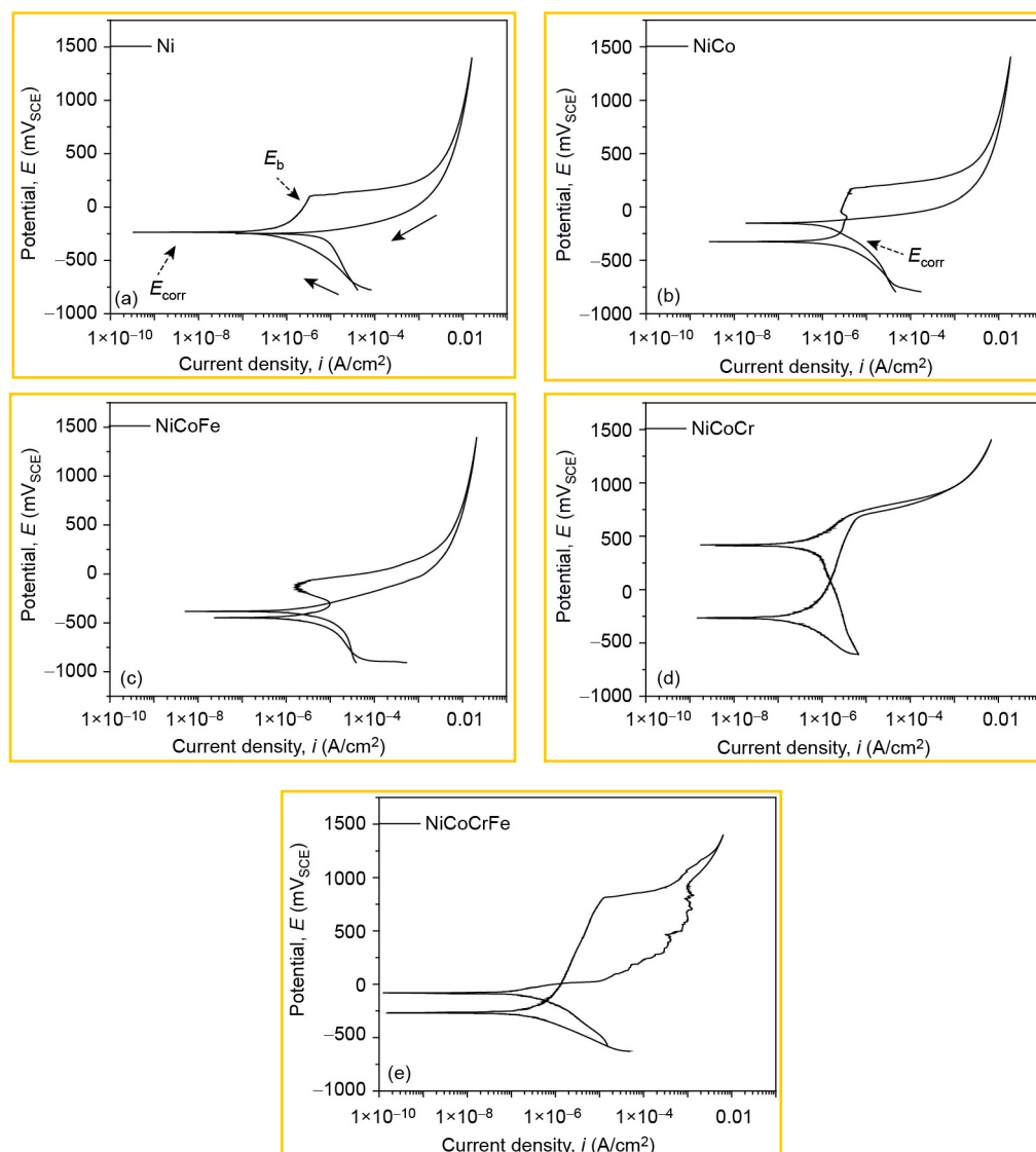
Figure 1 Cyclic polarization curves of alloys in 0.1 M NaCl. (a) Ni; (b) NiCo; (c) NiCoFe; (d) NiCoCr; (e) NiCoCrFe
